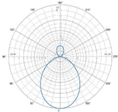
E-Plane | 405 MHz
