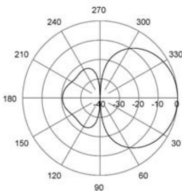
E-Plane | 104 MHz
