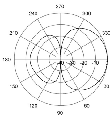
E-Plane | 50 MHz
