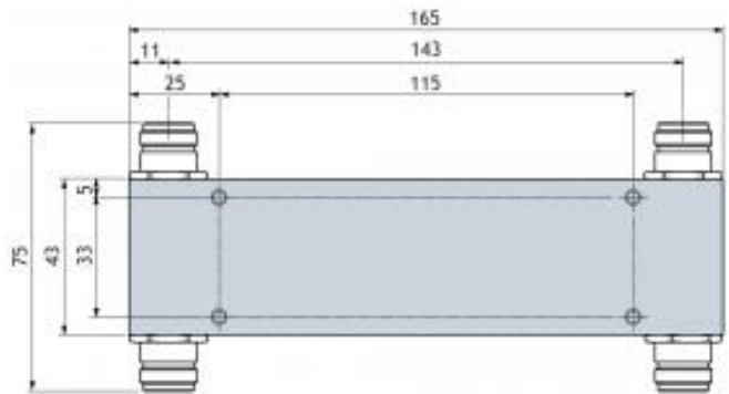
Mounting Details
