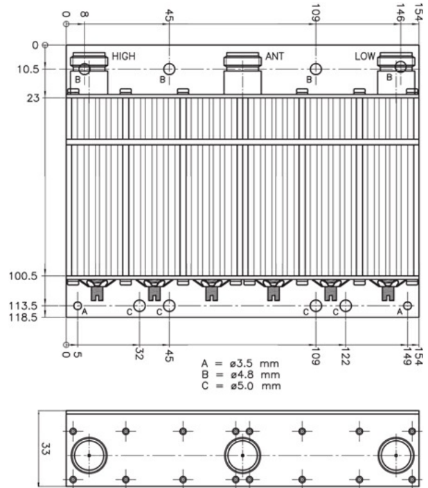
Mounting Details
