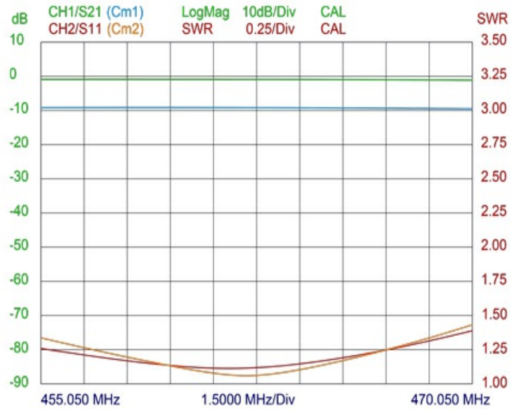
TYPICAL RESPONSE CURVE (10 DB VERSION)
