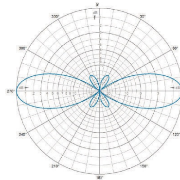
E-Plane | 875 MHz
