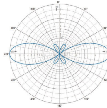
E-Plane | 395 MHz
