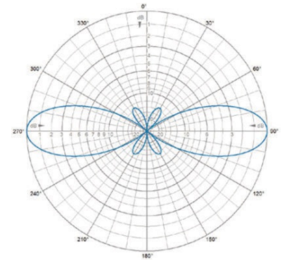
E-Plane | 340 MHz
