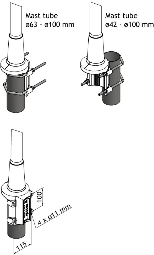
MULTI-PURPOSE MOUNTING BRACKET
