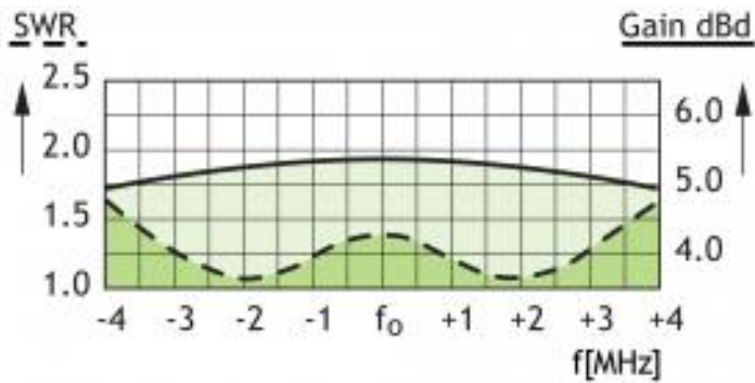
TYPICAL GAIN AND VSWR CURVES
