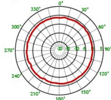
Typical Radiation Pattern for 300 MHz (H-Plane)
