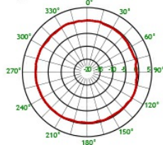
Typical Radiation Pattern for 350 MHz (H-Plane)
