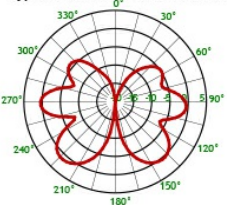
Typical Radiation Pattern for 400 MHz (E-Plane)
