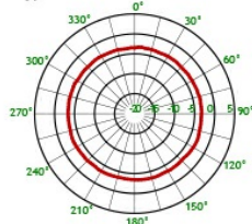
Typical Radiation Pattern for 250 MHz (H-Plane)
