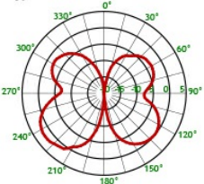
Typical Radiation Pattern for 250 MHz (E-Plane)
