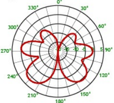
Typical Radiation Pattern for 350 MHz (E-Plane)
