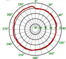
Typical Radiation Pattern for 400 MHz (H-Plane)
