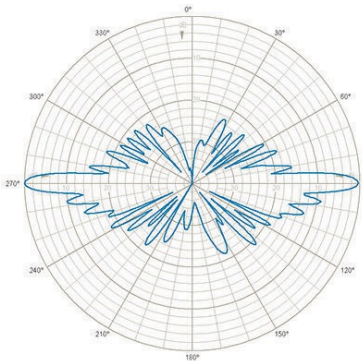
E-Plane | 875 MHz | 0°
