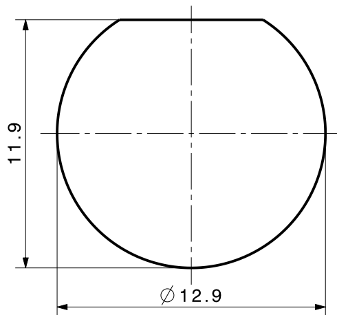
Mounting hole ML 4
