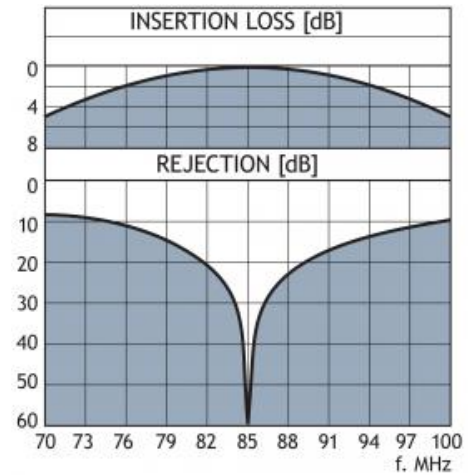
TYPICAL RESPONSE CURVE PRO-IS-85-S
