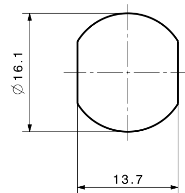
mounting hole (MH-12)
