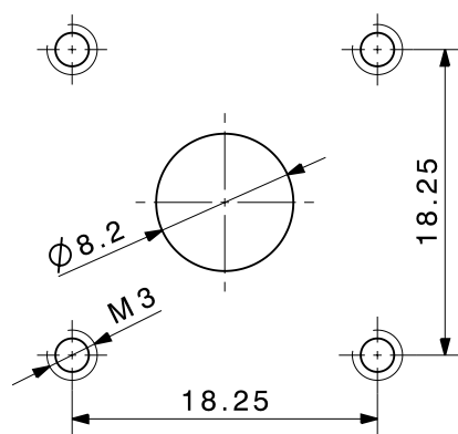
Front panel mount
