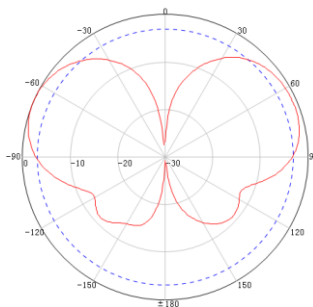
E PLANE
