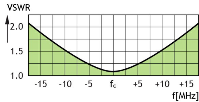
TYPICAL VSWR CURVE
