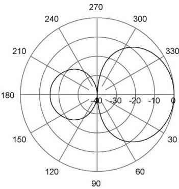
E-Plane | 102 MHz
