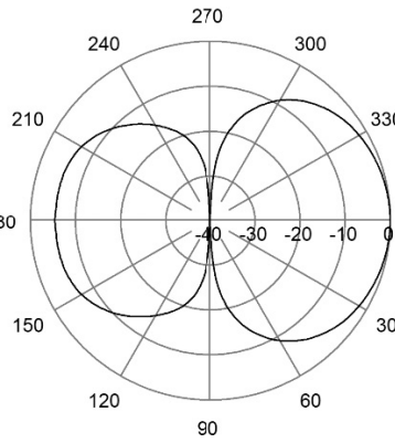
E-Plane | 98 MHz
