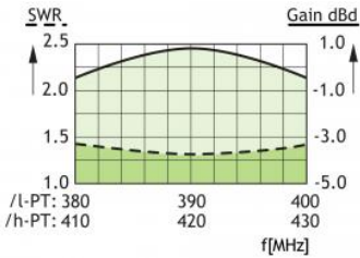
TYPICAL GAIN AND SWR CURVES
