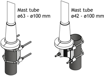
MULTI-PURPOSE MOUNTING BRACKET
