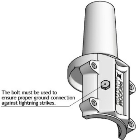
_X000D_ MOUNTING DESCRIPTION FOR GROUND CONNECTION
