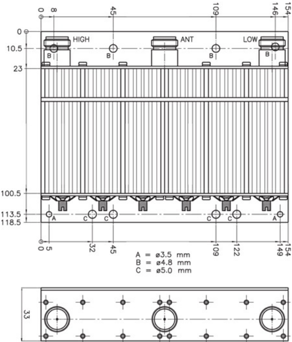
Mounting Details
