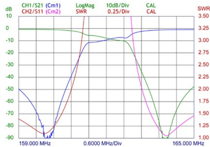
Typical response curves @ 5 MHz Duplex spacing
