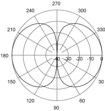
E-Plane | 426 MHz
