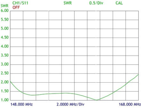
TYPICAL GAIN AND SWR CURVES
