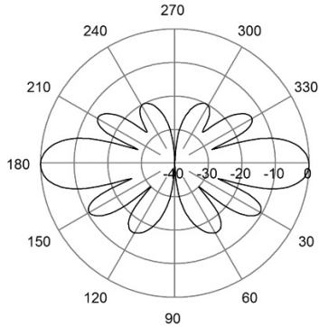
E-Plane | 910 MHz
