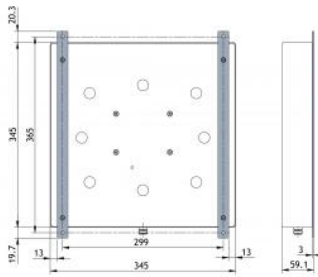
MOUNTING DETAILS (PATCH- WAMO)
