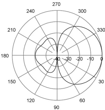
E-Plane | 435 MHz
