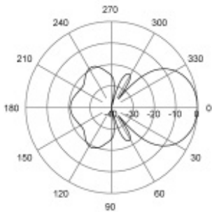
E-Plane | 875 MHz
