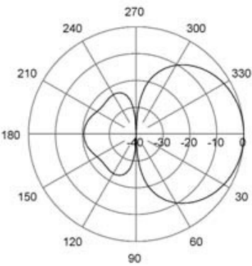
E-Plane | 72 MHz
