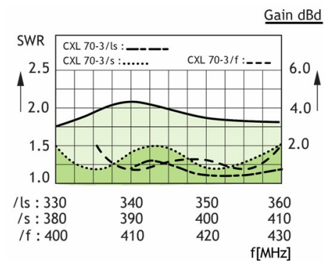
TYPICAL GAIN AND VSWR CURVES
