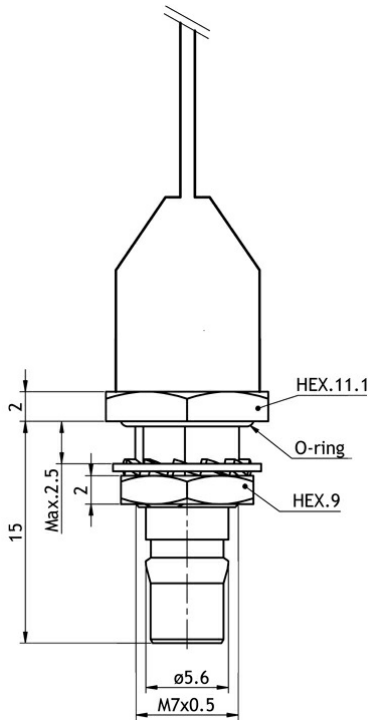
DIAGRAM MOUNTING DETAILS
