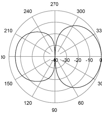
E-Plane | 405 MHz
