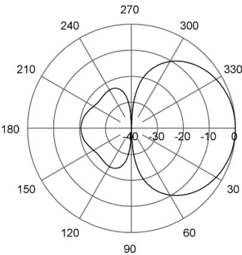
E-Plane | 405 MHz
