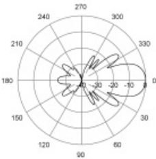
E-Plane | 435 MHz
