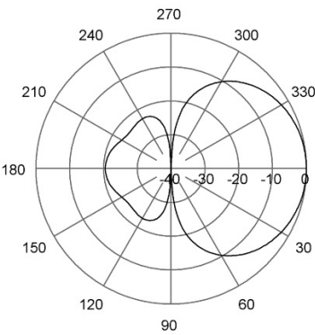
E-Plane | 82 MHz
