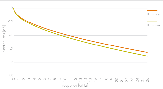
Insertion loss
