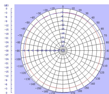
H Plane
