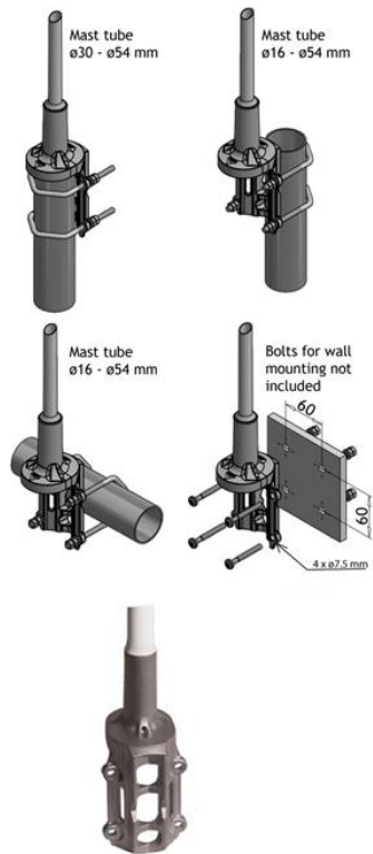
MULTI-PURPOSE MOUNTING BRACKET
