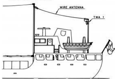
TYPICAL INSTALLATION:
