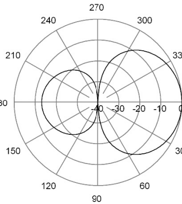
E-Plane | 73 MHz
