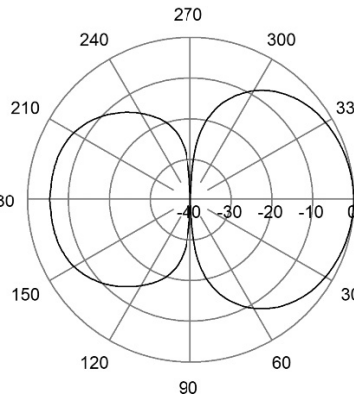
E-Plane | 68 MHz
