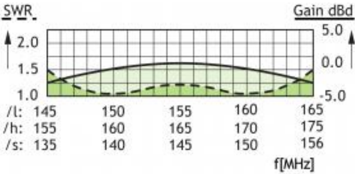
TYPICAL GAIN AND SWR CURVES
