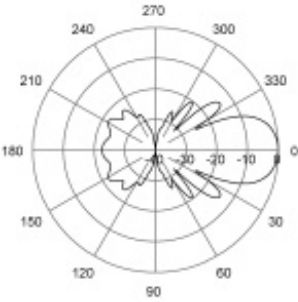
E-Plane | 580 MHz
