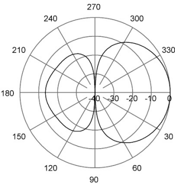
E-Plane | 72 MHz
