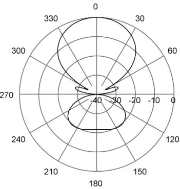
E-Plane | 110 MHz
