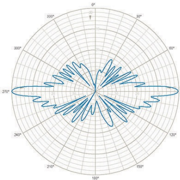
E-Plane | 875 MHz | 0°
