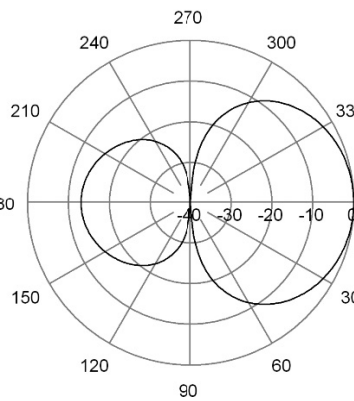
E-Plane | 98 MHz
