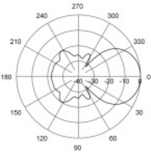
E-Plane | 395 MHz
