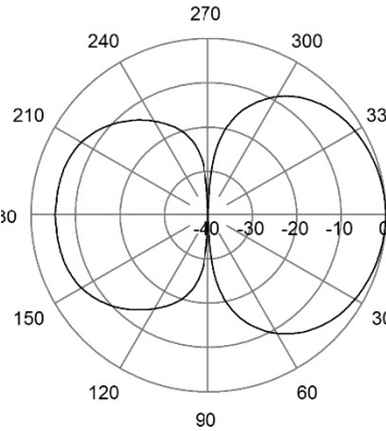
E-Plane | 459 MHz
