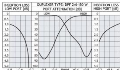
TYPICAL RESPONSE CURVES @ 1.6 MHz DUPLEX SPACING
