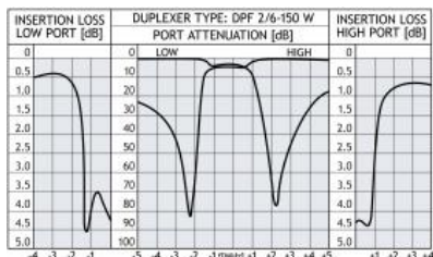
TYPICAL RESPONSE CURVES @ 4.5 MHz DUPLEX SPACING
